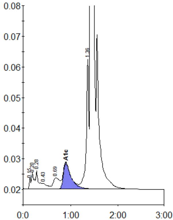
Peak table - ID: 10514001
